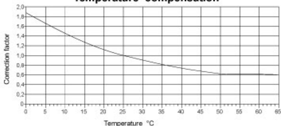
Temperature compensation
